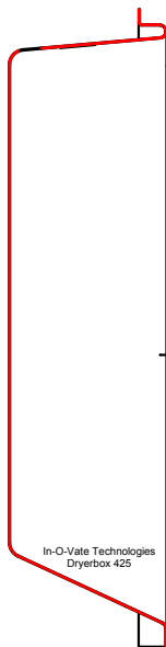
Sectional View
