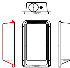
Sectional View SCALE 1/2
