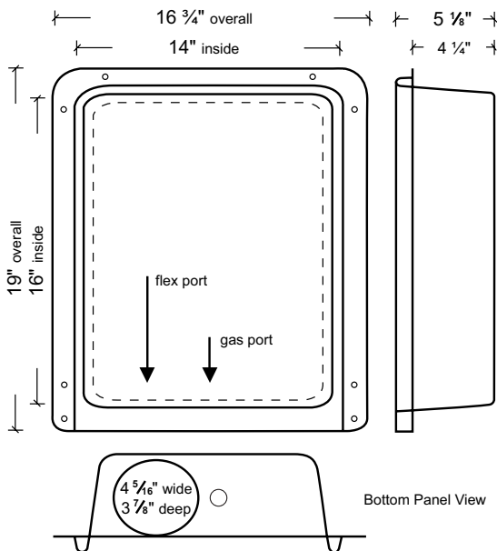
Recessed Dryer Vent Box MODEL 4D
