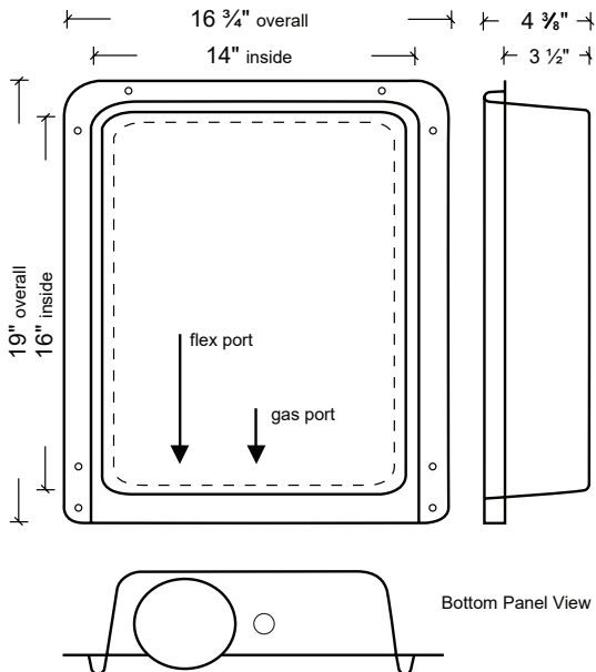
Recessed Dryer Vent Box MODEL 3D
